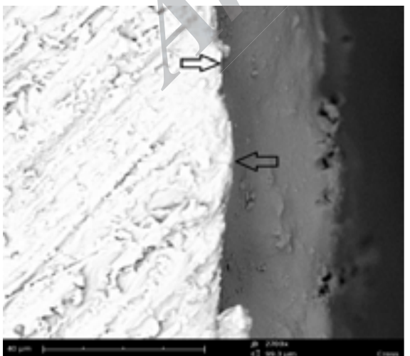
Figure 2: The cross-sectional view displaying the uniform junction. 20 \mu m thickness of coating (the coating is seen darker than the denture base).
