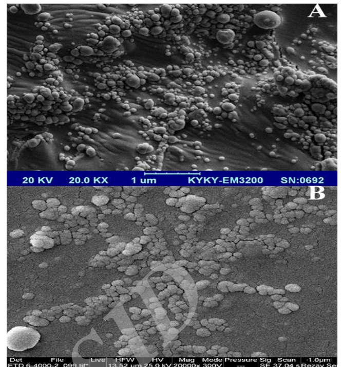
Fig.2. A) SEM micrograph of EVs preparations using ultracentrifugation method at 20Kx magnification. B) SEM micrograph of EVs preparations using PEG-based method at 20Kx magnification.
