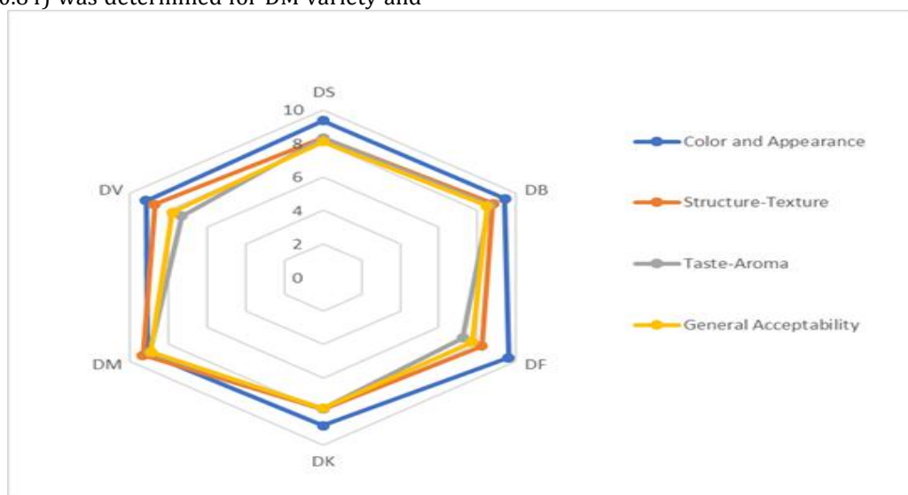
Figure 1. Sensory test scores for ice cream samples during storage. DS; control, DB; blackberry, DF; raspberry, DK; kiwi, DM; banana, DV; sour cherry (n=5x10).
