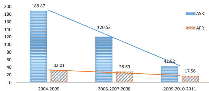
Figure 3. The average of Accident Frequency Rate (AFR) and Accident Severity Rate (ASR) indices in different years
