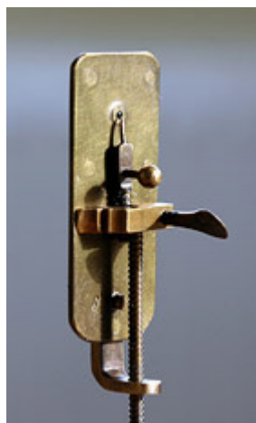
Figure 5. Anton Van Leeuwenhoek's Lens Grinding Device (2).
