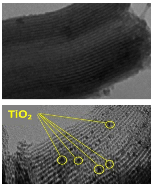
Fig. 3. TEM Images of the Synthesized CMK-3 and TiO 2 /CMK-3.
