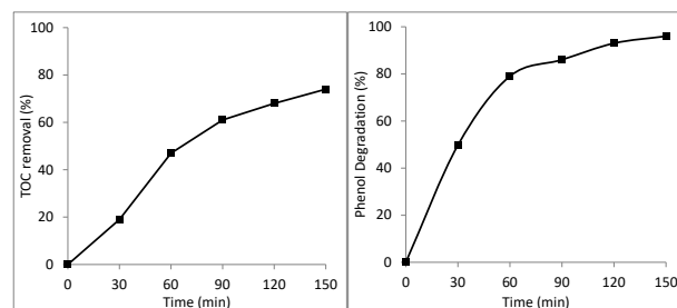
Fig. 8. Removal of TOC and Phenol During Photo-Catalytic Process (pH=6, TiO 2 /CMK-3 concentration=0.15 g/L, phenol concentration =100 mg/L)
