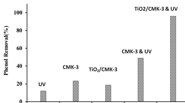
Fig. 4. Removal of Phenol Under Various Conditions (reaction conditions: pH= 6.0, catalyst (CMK-3 and TiO 2 /CMK-3) concentration = 0.15 g/L, phenol concentration =100 mg/L, and reaction time=150 min).
