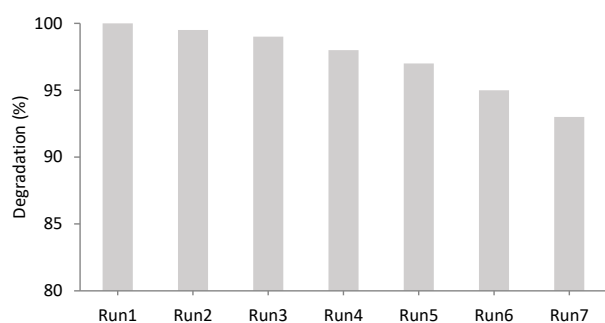
Fig. 9. Phenol degradation in consecutive runs using regenerated composite \text{TiO}_2/\text{CMK-3} as photo-catalyst (pH=6, concentration of \text{TiO}_2/\text{CMK-3}=0.15 g/L, phenol concentration=100 mg/L, and irradiation time=150 min)
