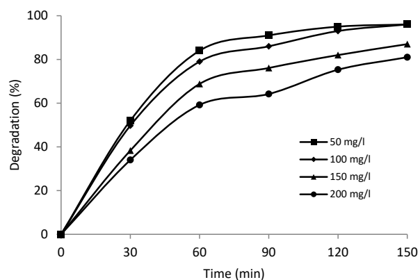
Fig. 7. Effect of initial concentration of phenol on the degradation efficiency of phenol (pH=6, concentration of TiO 2 /CMK-3=0.15 g/L, and irradiation time=150 min)
