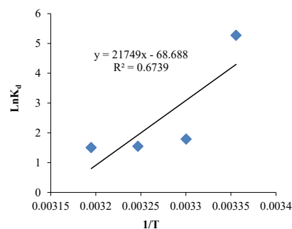
Figure 8. The Plot of the Adsorption of RB203 species onto Activated Carbon.
