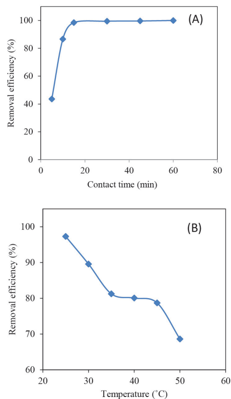
Figure 5. The Effect of Contact Time (A) and Temperature on the Removal of Dye (B)
