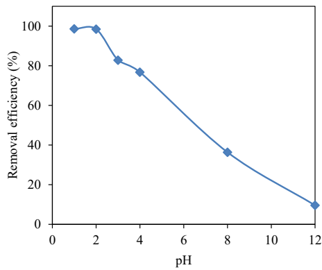
Figure 3. The Effect of pH on the Removal of RB203 by Activated Carbon.
