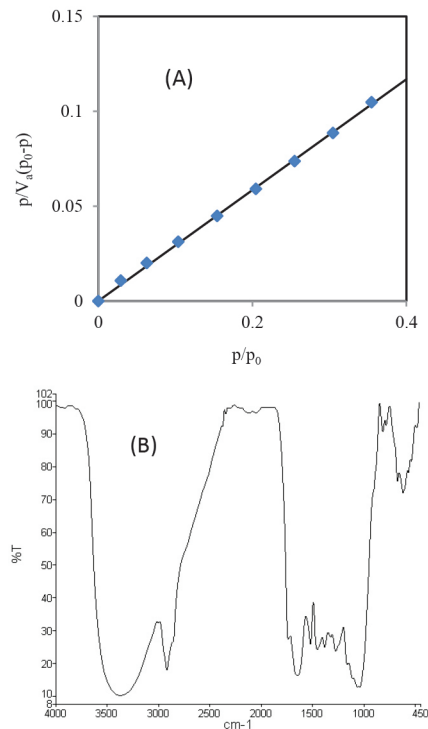
Figure 2. BET Plot of \text{N}_2 Adsorption-desorption Isotherms of Pure Activated Carbon (A) and FT-IR Spectra Related to Activated Carbon from Pine Cones (B).
