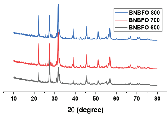
Fig. 1. XRD Results of BNBFO Nanoparticles Annealed at 600, 700 and 800°C.
