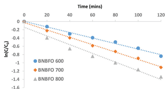
Fig. 6. MB Photodegradation and the First-order Kinetics.
