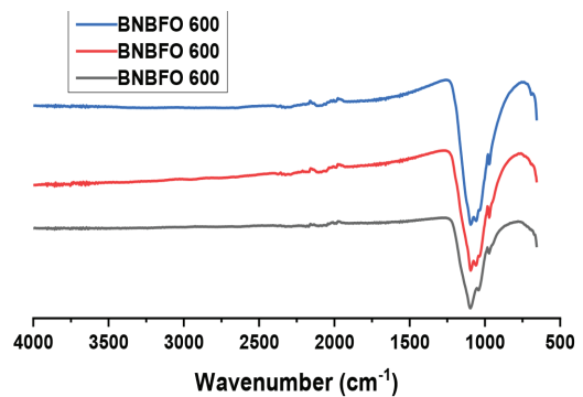
Fig. 3. FTIR Results of BNBFO Nanoparticles Annealed at 600, 700 and 800°C
