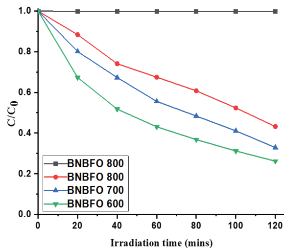
Fig. 5. Photocatalytic results of BNBFO Nanoparticles Annealed at 600, 700 and 800°C.
