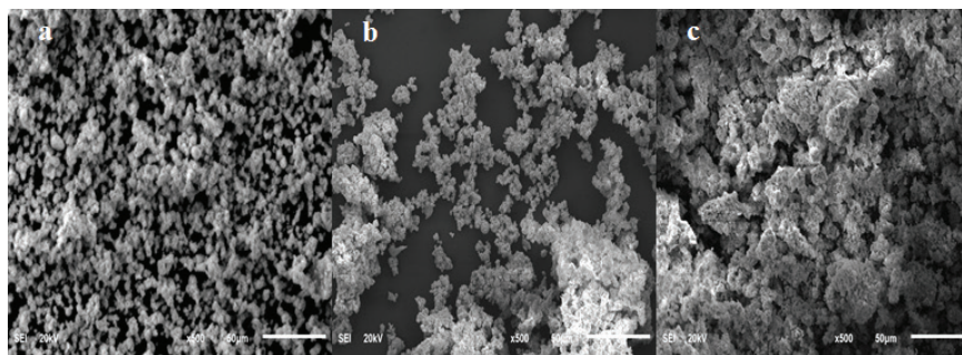
Fig. 2. SEM image of BNBFO Nanoparticles Annealed at 600, 700 and 800°C
