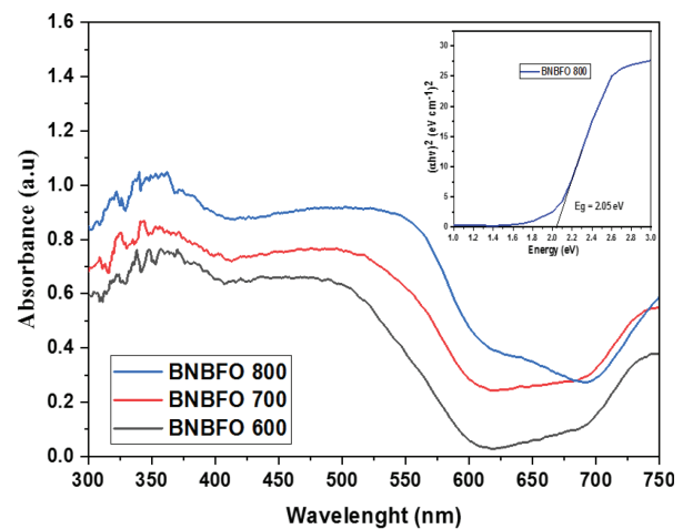
Fig. 4. DRS results of BNBFO Nanoparticles Annealed at 600, 700 and 800°C.
