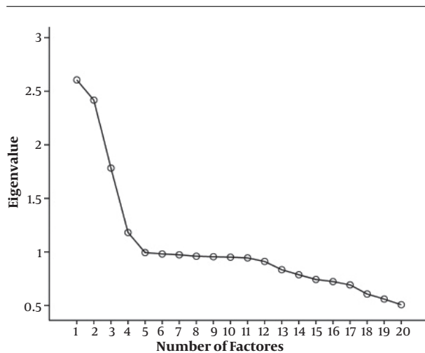
Figure 1. Scree Plot of Eigenvalue
