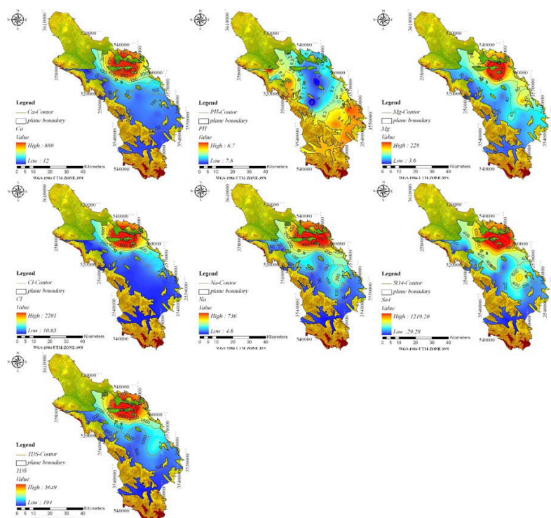
Figure 3. Interpolate drinking water parameters by kriging method.
