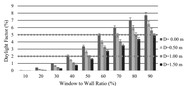
Figure 3. Amount of daylight factor in different models with different WWR according to the depth of overhang
