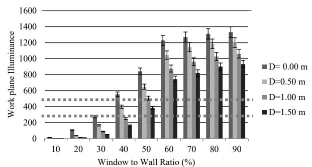
Figure 4. Amount of work plane illuminance in different models with different WWRs according to the depth of overhang
