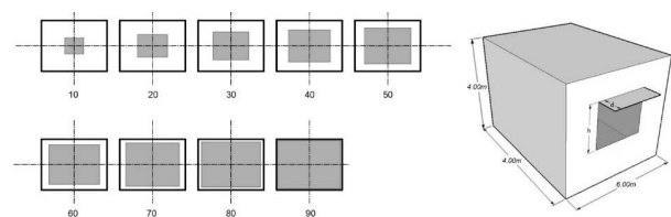
Figure 2. Window size variations of office rooms with different overhang depths.
