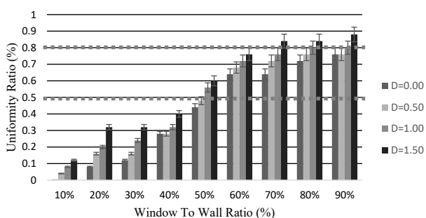
Figure 5. Amount of uniformity ratio in different models with different WWRs according to the depth of overhang.
