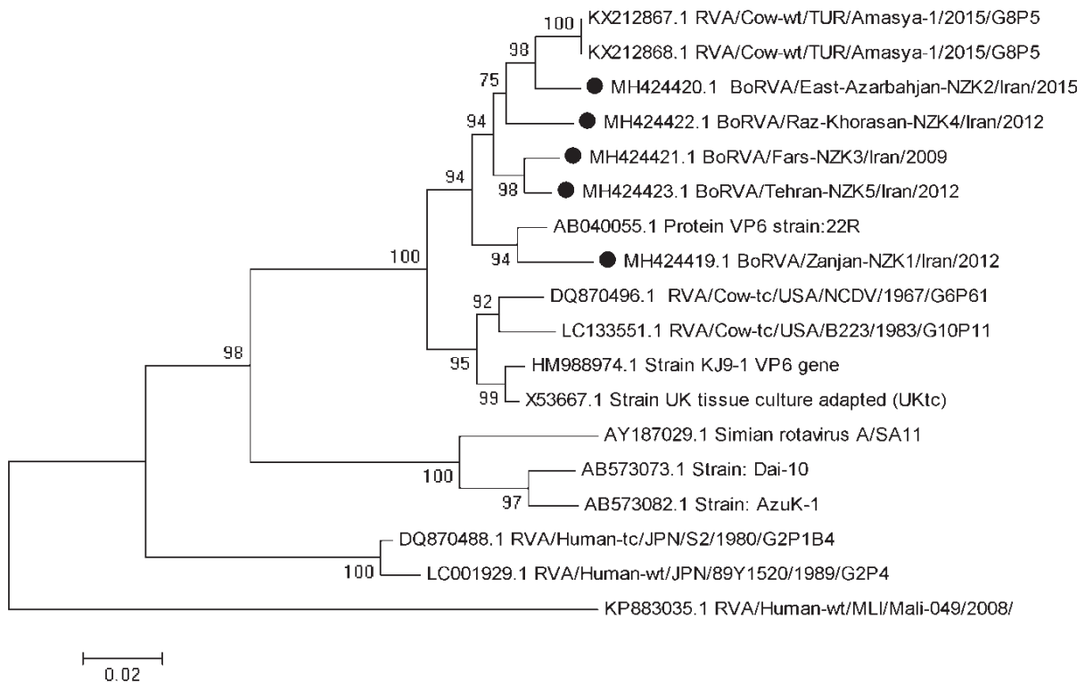
Figure 1. The Evolutionary History of the Nucleotide Sequence of the VP6 Gene of bovine RVA circulating in Iran.
