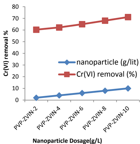
Fig.5. The removal efficiency of Cr(VI) using PVP-ZVINS as a function of PVP- ZVINS dosage
