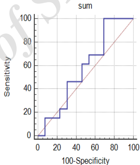
Figure 5: Roc curve
