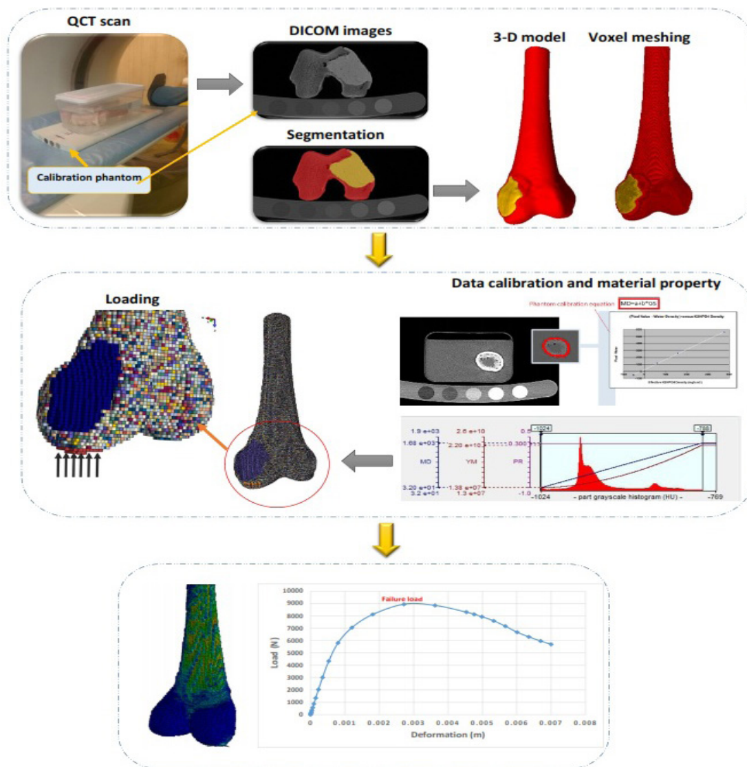
Figure 1. Various steps taken in making a voxel based finite element (FE) model of a long bone affected by GCT. The specimen is first scanned by QCT, in which a calibration phantom is used during the scanning procedure. DICOM images are imported into 3D modeling software for segmentation of the desired bones or parts. The 3D model is then meshed based on the QCT voxels. Using the calibration equation derived from known phantom tubes densities, as well as relations available in the literature for converting densities into mechanical properties, material properties can be assigned to each voxel of the model. Desired boundary and loading conditions are applied to the model, and the results in the form of stress, strain, and failure load can analyzed.
