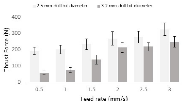
Figure 3. Thrust force versus six different feed rates for 2.5 and 3.2 mm drill bit diameters.
