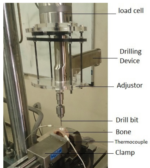
Figure 1. Set up for the drilling process and recording thrust force and temperature versus time for each bone sample.
