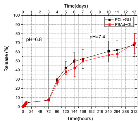
Figure 7. In vitro release studies of GLI from PCL and PBAd MPs
