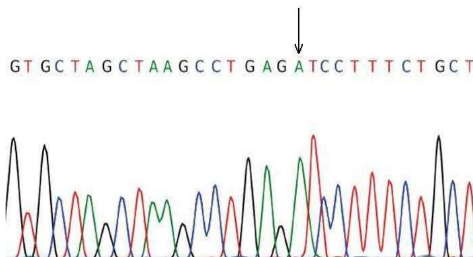
Fig. 5. Hemizygous mutation of exon 12
