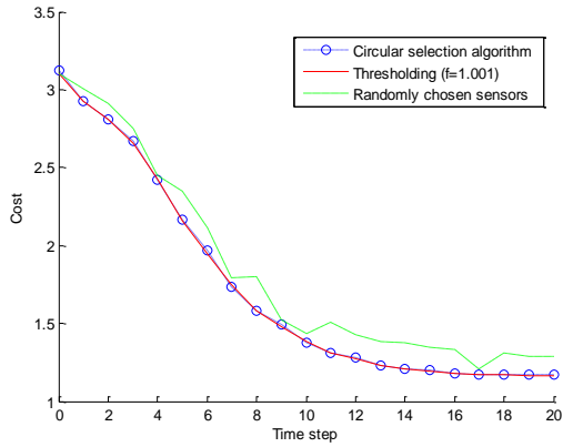
Figure 3: Comparison between circular selection, thresholding, and randomly chosen algorithms.
