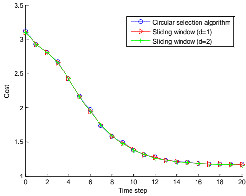
Figure 4: Comparison between circular selection, sliding window (d=1), and sliding window (d=2) algorithms.
