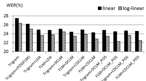
Fig. 4. WERs of combination LMs with acoustic model
