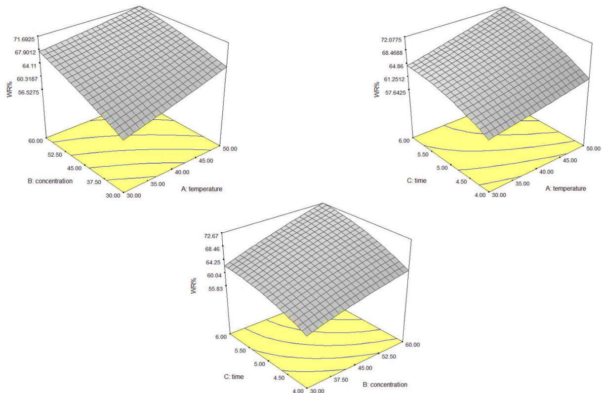
Fig. 3. The interaction effect of the independent variables of osmotic solution temperature - osmotic solution concentration - osmotic solution temperature - immersion time and osmotic solution concentration - immersion time on WR (%) of turnip slices
