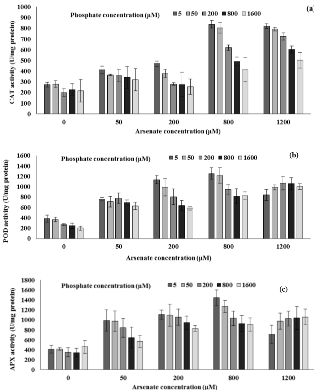
Figure 6. Catalase (a), peroxidase (b) and ascorbate peroxidase (c) activity (U mg protein -1 ) in I. cappadocica grown for 4 weeks in arsenate and phosphate amended medium. The data are means ± S.D for 3 individual measurements in each group.
