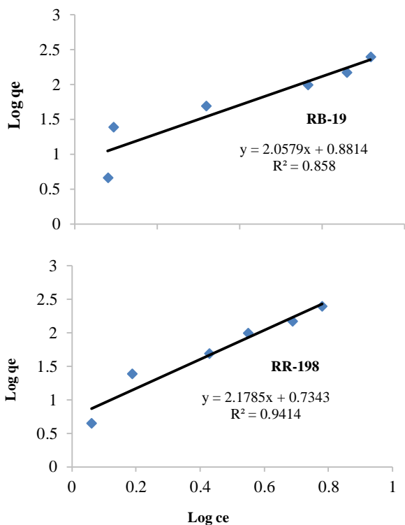
Fig.7. Freundlich adsorption isotherms of RR198 and RB19 on Acaciatortilis plant shuck to mesh size 30-60
