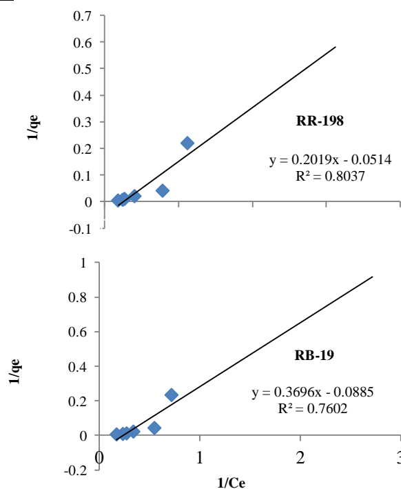
Fig.6. Langmuir adsorption isotherms of RR198 and RB19 on Acaciatortilis plant shuck to mesh size 60-100
