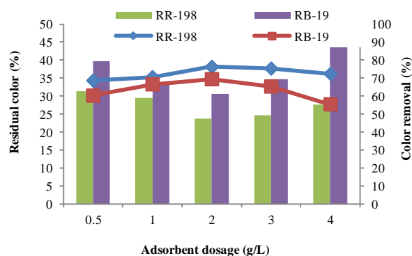
Fig.2. Effect of adsorbent dosage on adsorption of the dye by Acaciatortilis plant shuck. Conditions: 50 mg/L Concentration of dye, 30 minutes contact time, pH 4
