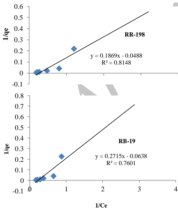
Fig.5. Langmuir adsorption isotherms of RR198 and RB19 on Acaciatortilis plant shuck to mesh size 30-60
