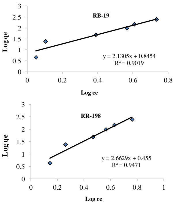
Fig.8. Freundlich adsorption isotherms of RR198 and RB19 on Acaciatortilis plant shuck to mesh size 60-100
