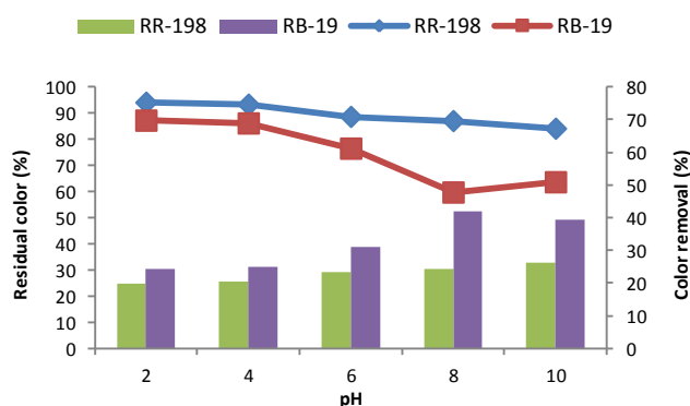
Fig.1. Effect of pH on adsorption of the dye by Acaciatortilis plant shuck. Conditions: 50mg/L concentration of dye, 30 minutes contact time, 1g/L adsorbent dosage
