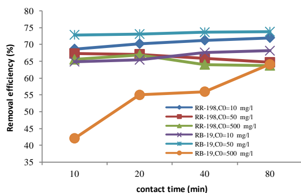
Fig.3. Effect of contact time and initial dye concentration on adsorption of the dye by Acaciatortilis plant shuck. Conditions: pH 4, 2 g/L adsorbent dosage, mesh size 30-60
