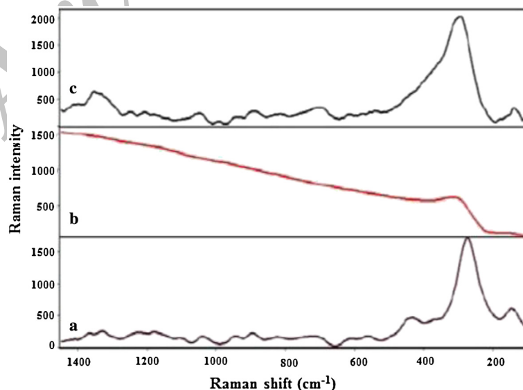
Figure 4 Raman spectra and SERS of \text{Nd}_2\text{O}_3 molecules using colloidal silver. The Raman spectrum of 1M \text{Nd}_2\text{O}_3 solution (a). The Raman spectrum of 0.01 M \text{Nd}_2\text{O}_3 solution (b). The SERS spectrum of 0.01 M \text{Nd}_2\text{O}_3 by silver colloid (c).
