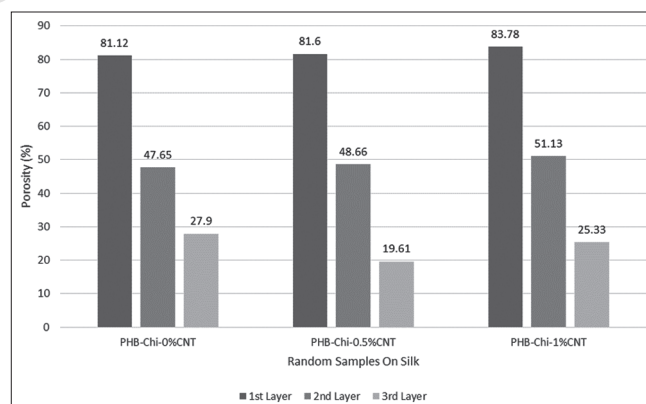
Figure 3: Porosity percentage charts of nano-micro scaffolds in three layers
