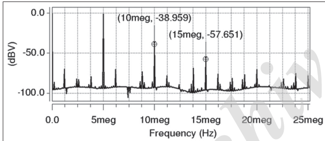
Figure 5: The fast Fourier transform results for the inverter-based operational transconductance amplifier circuit
