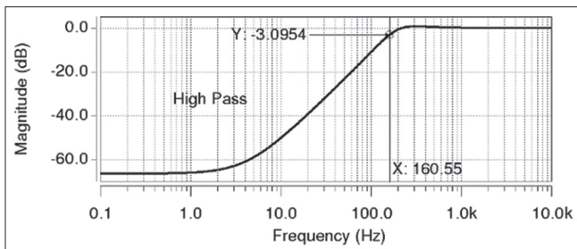
Figure 11: Frequency response for the proposed filter in the high-pass mode
