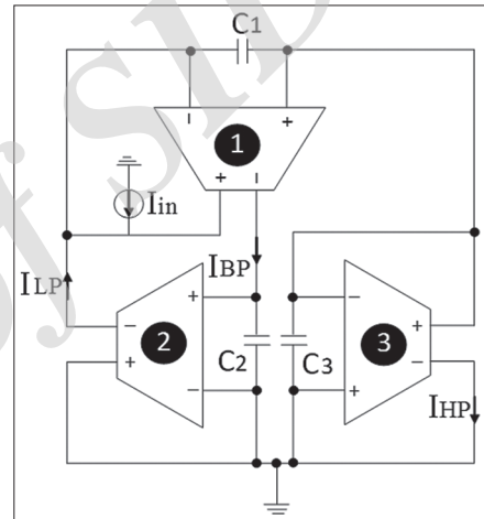
Figure 3: The proposed third-order universal operational transconductance amplifier-capacitor filter
