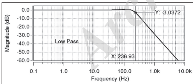
Figure 9: Frequency response for the proposed filter in the low-pass state
