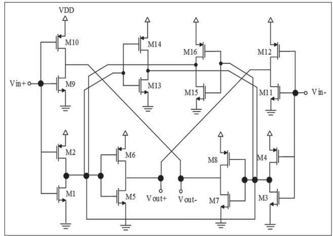
Figure 2: The inverter-based transconductance circuit used in the operational transconductance amplifier-capacitor filter
