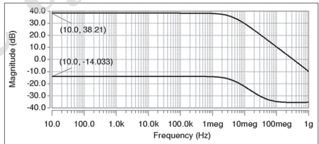
Figure 6: Common-mode rejection ratio obtained for the inverter-based circuit
