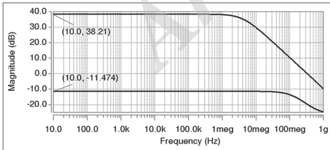
Figure 7: Power supply rejection ratio obtained for the inverter-based operational transconductance amplifier circuit
