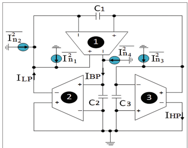
Figure 4: Circuit model used to study noise in the proposed third-order current-mode universal operational transconductance amplifier-capacitor filter
