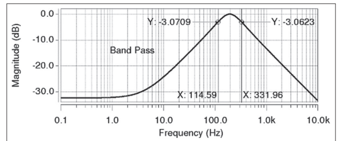
Figure 10: Frequency response obtained for the proposed filter in the band-pass state
