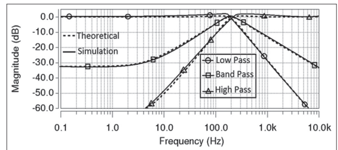
Figure 12: Comparison between theoretical and simulation results obtained for the proposed filter
