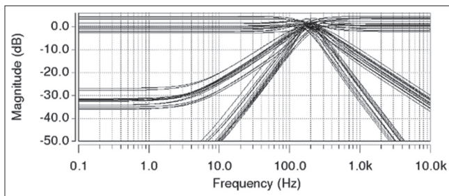
Figure 13: Monte Carlo analysis results obtained for the frequency responses of the proposed filter
