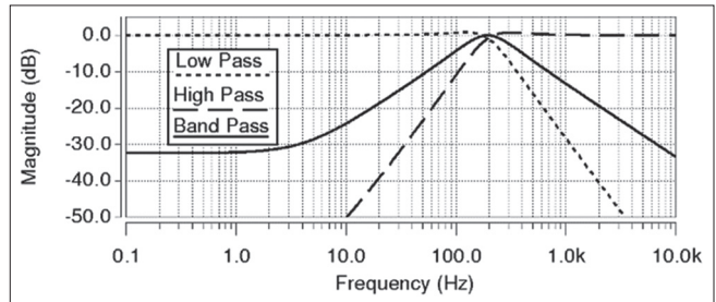
Figure 8: The frequency response obtained for the proposed filter
