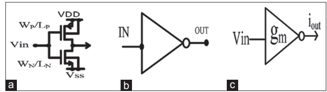
Figure 1: The different symbols used for inverters : a) showing a particular type of inverter; b) a more common representation and c) transconductance inverter
