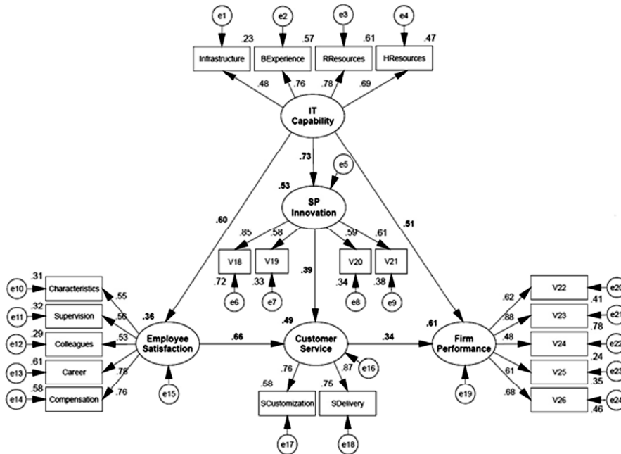
Fig. 2. Accepted SEM along with standardized coefficients
