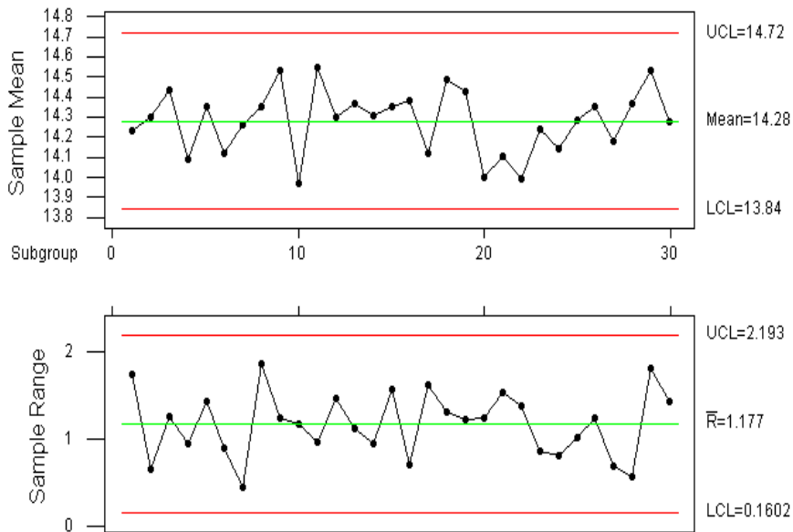
Fig. 10. \bar{X} and R Control Charts After the Calibration (Made With Minitab Software)
