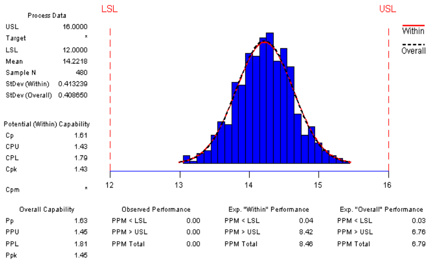
Fig. 17. Process Capability Indices (Created With Minitab Software)
