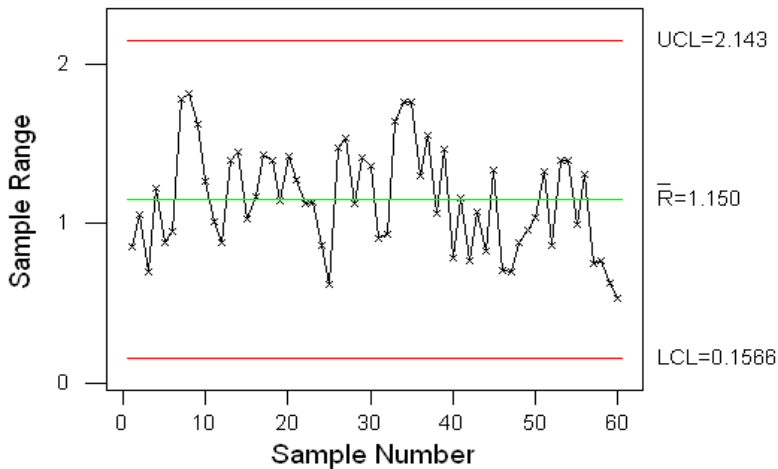
Fig. 13. R Control Chart (Created With Minitab Software)
