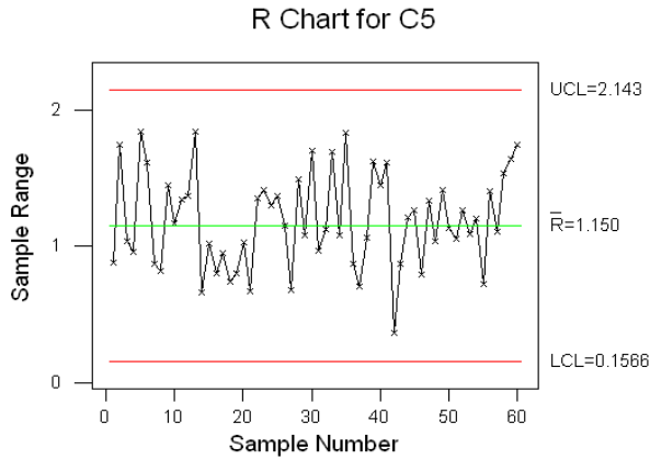
Fig. 16. R Control Chart (Created With Minitab Software)
