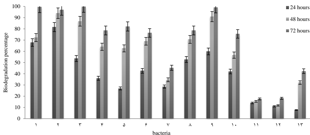
Fig. 3- Biodegradation percentages of tannic acid (15 g/l) after 24, 48 and 72 h of incubation; (1- 7: bacterial isolates from goat feces after feeding on tannin rich diet, 8, 9: before feeding on tannin rich diet and 10- 13: bacterial isolates from P- SH).
