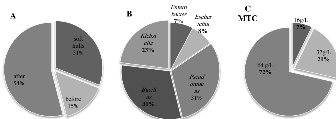
Fig. 2- Percentage of isolated bacteria according to source of isolation (A), identified genus (B) and Maximum Tolerable concentration of Tannin (C).
