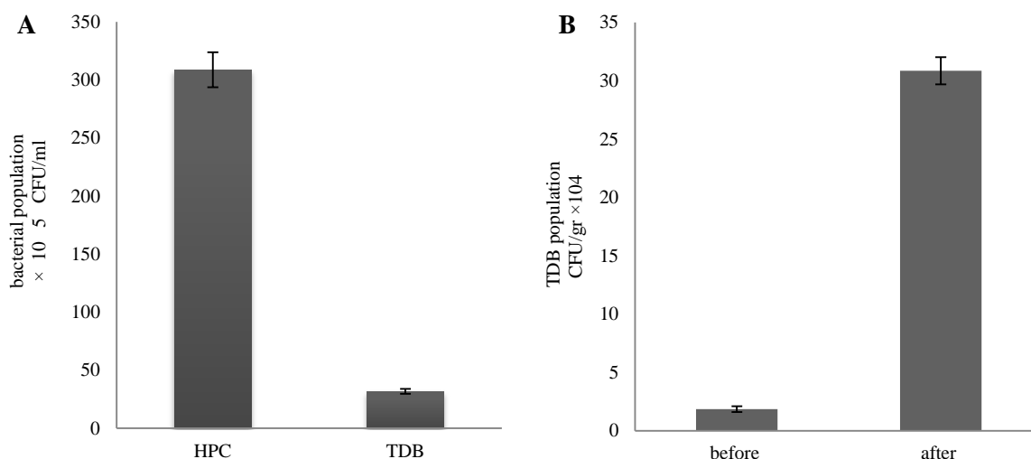
Fig. 1- Heterotrophic and Tannin degrading bacteria (TDB) of P- SH (A).TDB population of goat feces before and after feeding on tannin rich diet (B).
