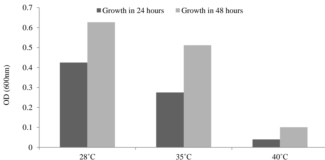
Fig. 3- Growth rate of isolates based on OD in different temperatures
