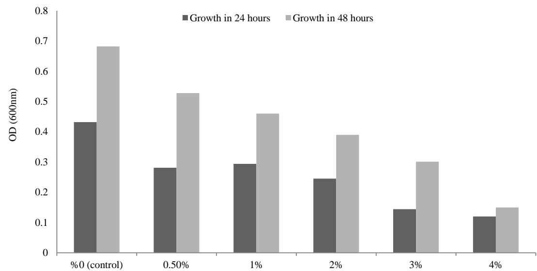
Fig. 1- Growth rate of isolates based on OD in the presence of different concentrations of NaCl in YEMB
