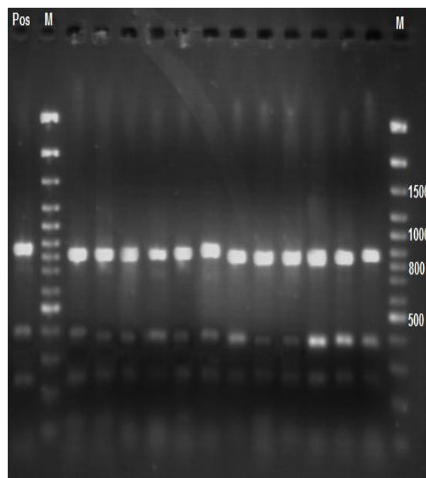
Fig. 5- TaqI digestion pattern of PCR products of S. meliloti isolates
