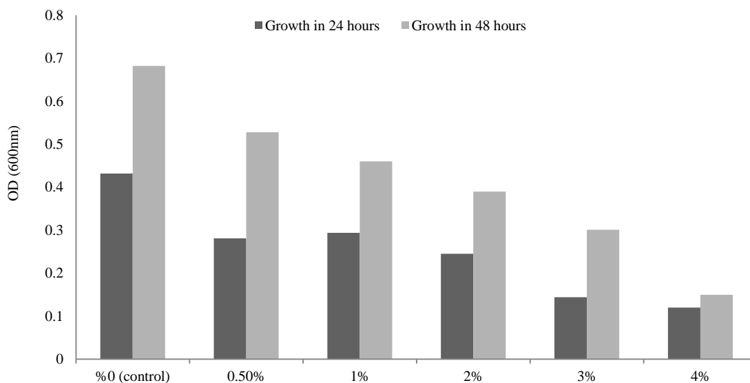
Fig. 1- Growth rate of isolates based on OD in the presence of different concentrations of NaCl in YEMB
