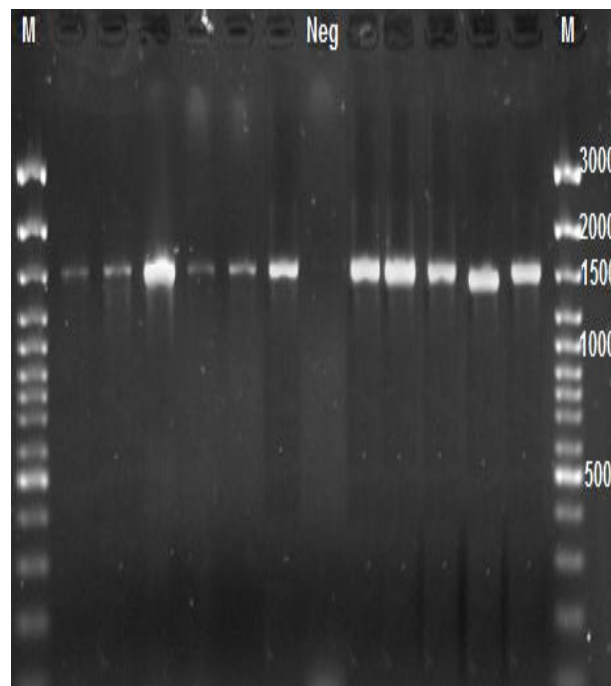
Fig. 4- Gel electrophoresis of 16S rDNA gene PCR product of Sinorhizobium isolates by rD1 and fD1 primers (M: marker, Neg: negative control)
