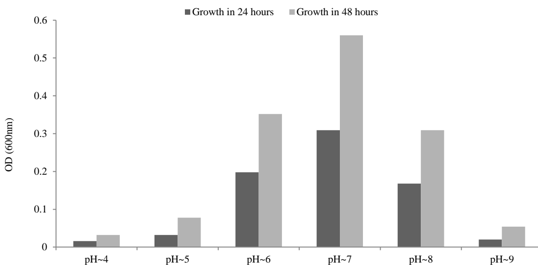
Fig. 2- Growth rate of isolates based on OD in media with different acidities
