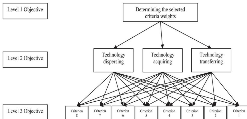
Figure2: Decision hierarchical the for determining the relative importance of choices
