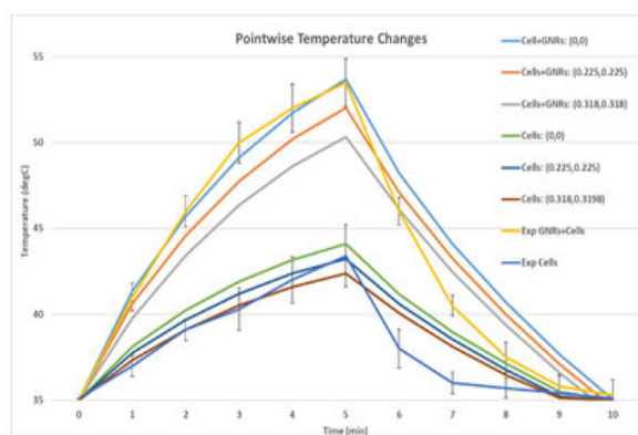
Figure 7: Temperature curve of three points with different distances from center of the illuminated well in our simulated cell-culture-plate. (green: center; blue: r=0.3 cm; red: r=0.45 cm) for Cells+gold nanorods (GNRs) and Cells separately compared to experiment (Exp).
