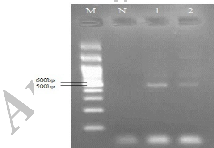
Figure 3 Agarose gel electrophoresis of PCR products amplified with Fsc1 EF1/Fsc1 EF2 primers (race 1 specific primers). M, 1kb ladder, N, negative control, line 1 and 2 studied isolates.
