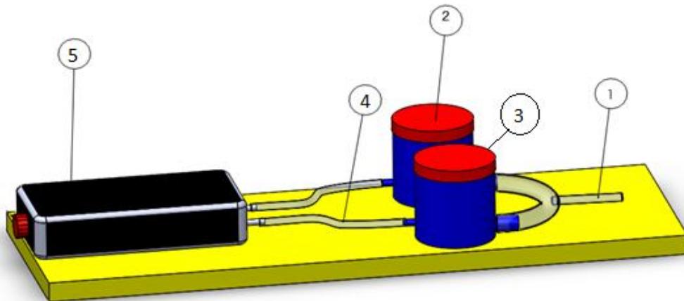
Figure 1 Schematic figure of Y-shaped olfactometry device (1. Common entrance tube, 2 and 3. Sample chamber, 4. Connective tube, 5. Electric engine to create airflow).
