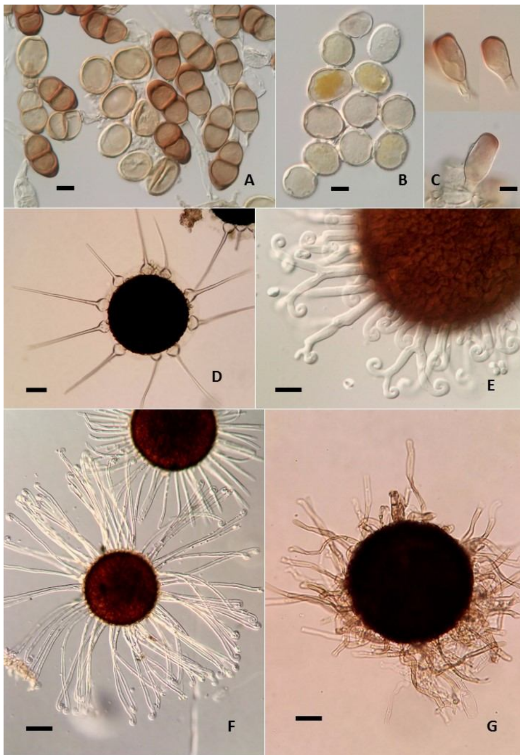
Figure 1 Puccinia tanacetii , urediniospores and teliospores, bar = 10 \mu m (A); Uromyces dactylidis , urediniospores (B) and teliospores (C), bar = 10 \mu m; Phyllactinia corni , chasmothecium (D), bar = 50 \mu m; Sawadaea bicornis , chasmothecium (E), bar = 15 \mu m; Erysiphe adunca , chasmothecia (F), bar = 60 \mu m; Golovinomyces asterum var. solidaginis , chasmothecium (G), bar = 30 \mu m.
