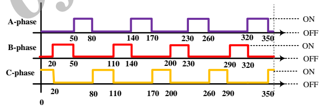
Fig. 12. Ripple torque switch timing
