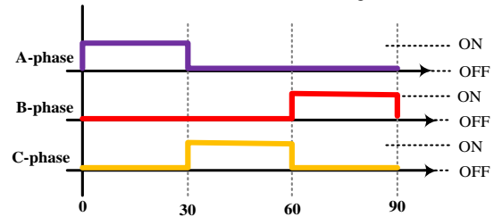
(b) Drive switched timing chart (rotation angle (deg.))
