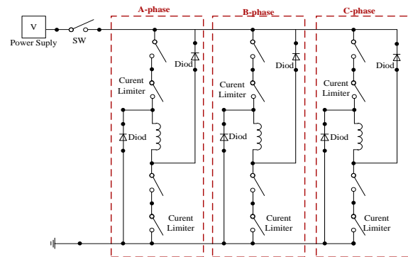
(a) Drive circuit diagram
