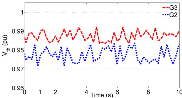
Fig. 11. Thévenin voltage in case of load rejection
