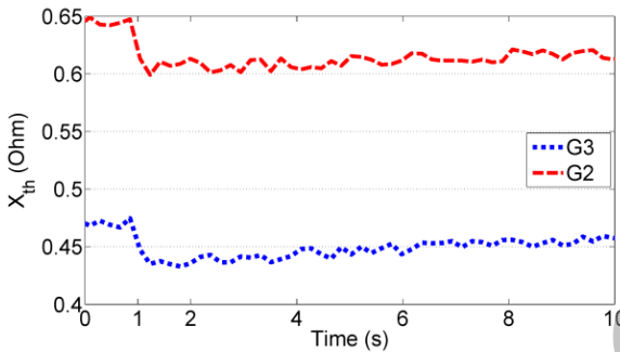
Fig. 9. Thévenin impedance in case of load entrance
