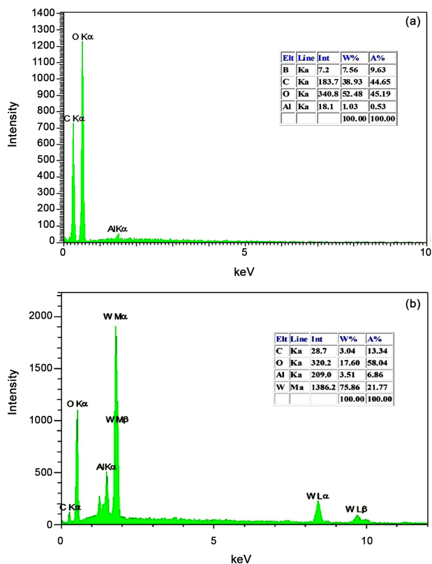
Fig. 3. EDS analysis of: (a) \text{Al}_2(\text{B}_4\text{O}_7)_3 -coated fiber and (b) \text{Al}_2(\text{WO}_4)_3 -coated fiber.
