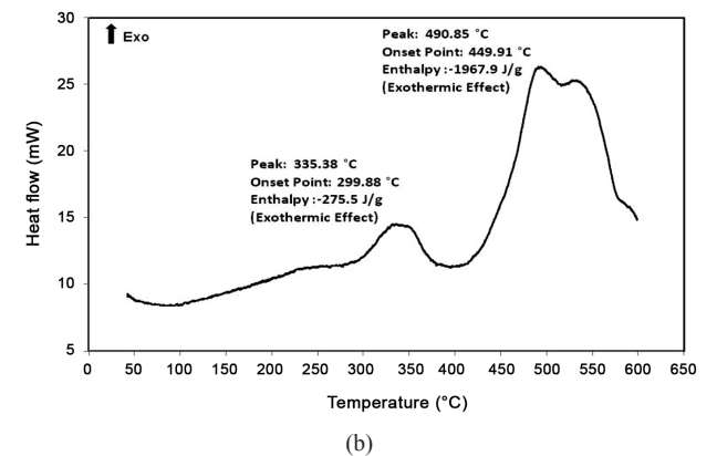
Fig. 8. TGA/DTG and DSC curves of Al 2 (WO 4 ) 3 treated cellululosic fiber.
