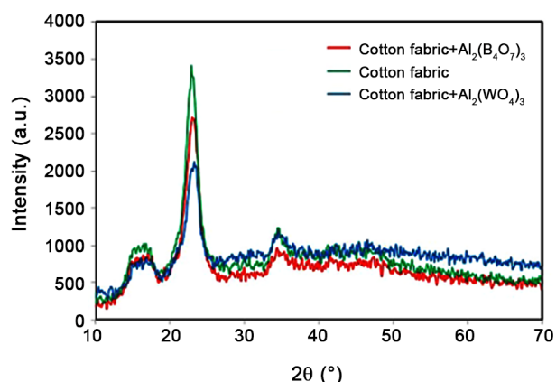
Fig. 5. XRD patterns of pure cellulosic fibers and flame retardant nanocomposite fibers.
