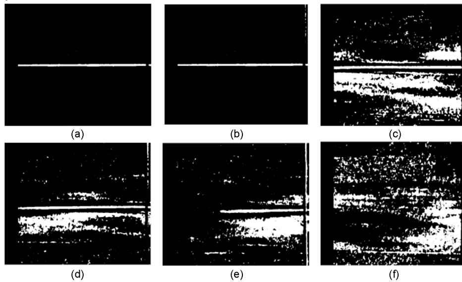
Fig. 7. Images extracted from online video frames after thresholding: (a) frame contains weft yarn, (b) frame contains weft yarn and warp yarn, (c) frame contains weft yarn, warp yarn, reed loom and rapier, (d) frame contains weft yarn, warp yarn, reed loom, and rapier, (e) frame contains weft yarn, warp yarn, reed loom, and rapier, and (f) frame contains weft yarn, warp yarn, reed loom, and rapier.
