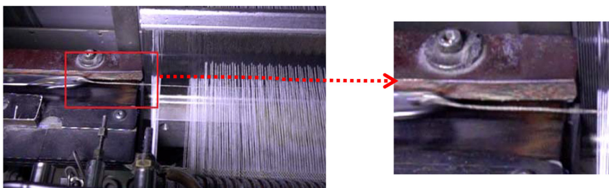
Fig. 4. Selected region covering the rapier exit and the selvedge weft yarn.
