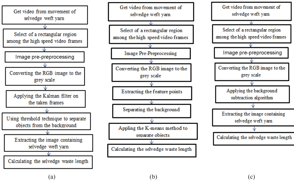
Fig. 3. Flowchart of proposed methods for calculating the selvedge yarn length: (a) based on Kalman filter, (b) based on K-means, and (c) based on background subtraction.
