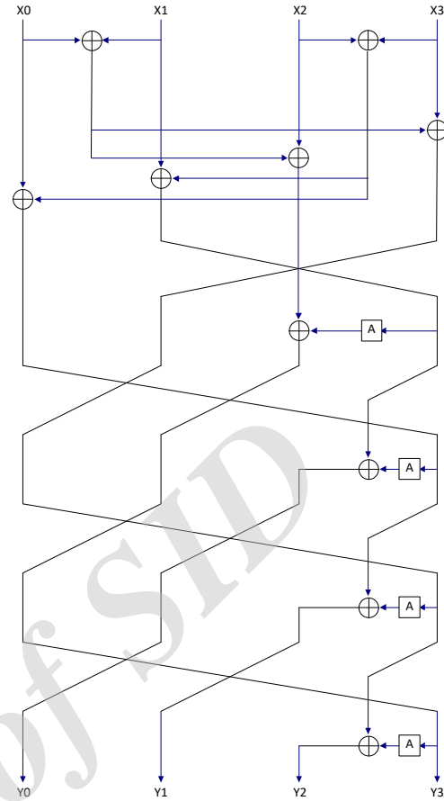
Figure 1. The corresponding diffusion layer of (2)
