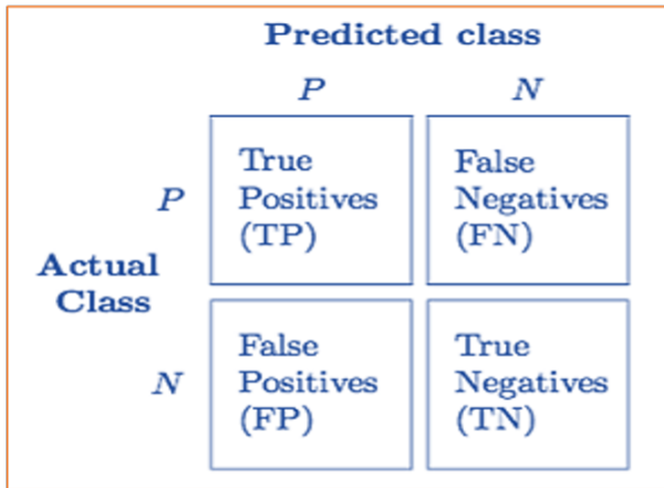
Figure 9. confusion matrix
