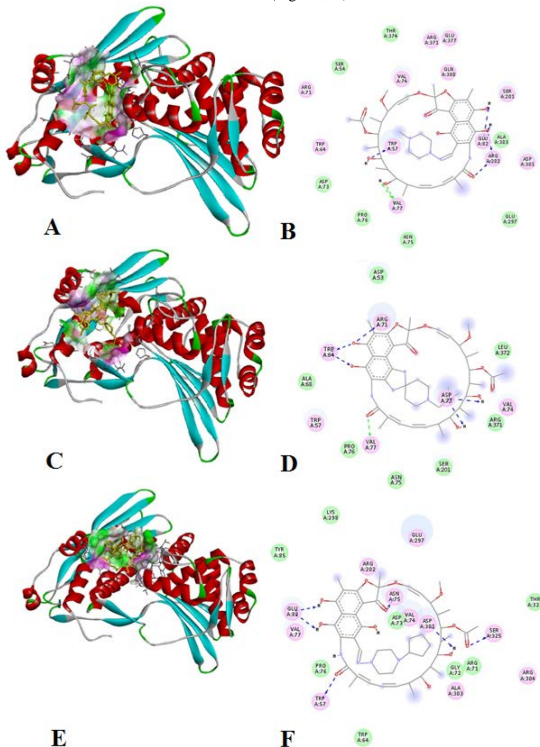
Figure 5: Molecular interaction of modelled rpoB with drug molecules (A, B: with rifampicin, C, D: with rifabutin, E, F: with rifapentine)
