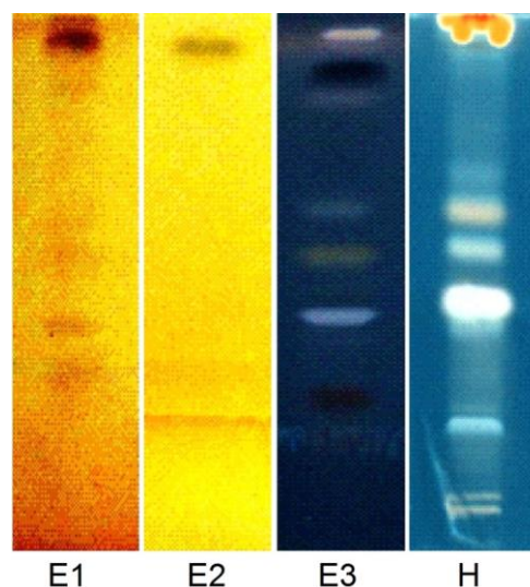
Figure 1. HPTLC fingerprints of S. securidaca seeds oil fractions run in different mobile phases (MP) and treated with, orcinol (E1), \text{FeCl}_3 (E2) and Liebermann-Burchard (E3, H). E1, E2 and E3: ethanol fraction run in MP3; H: fixed oil run in MP4
