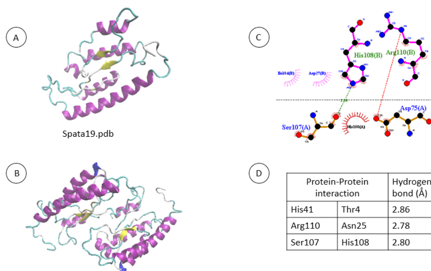
Figure 6. Modeling and docking of Spata19 and mGpx4
