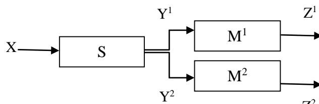
Figure 1. A Two-Stage Supply Chain with one supplier and two manufacturers.
