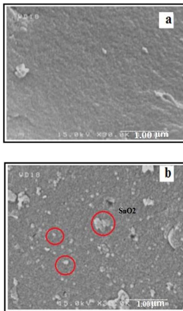
Fig.4. SEM images for (a) AC and (b) SnO 2 /AC.
