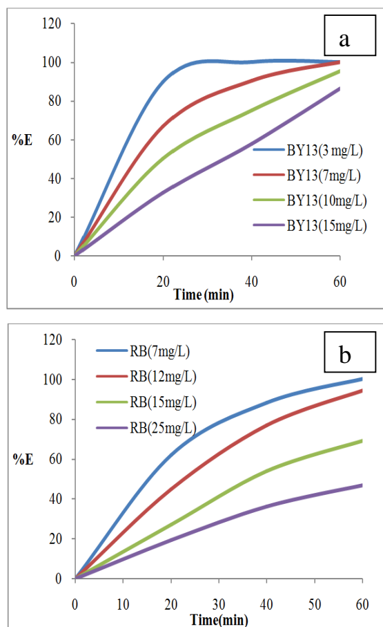
Fig.7. Effect of initial dye concentrations on degradation efficiencies of (a) BY13 and (b) RB.
