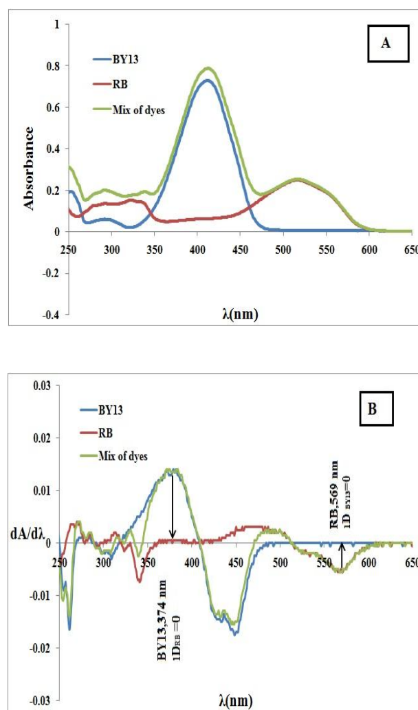
Fig.1. (A) Zero-order absorption spectra and (B) first-order absorption spectra for BY13 and RB in single and binary dye solutions, respectively.
