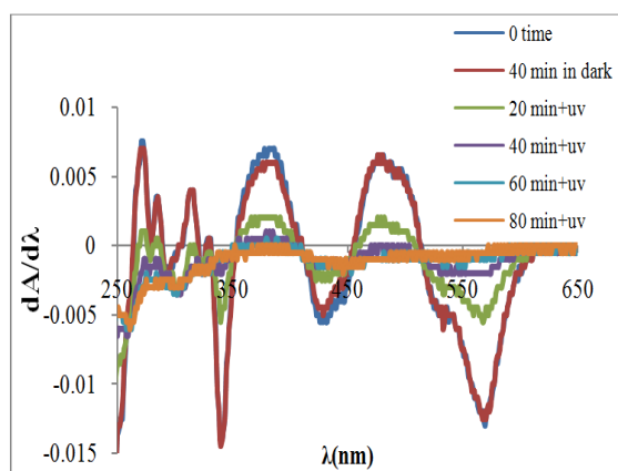
Fig.5. First-order absorption spectra for MO solution as a function of UV light exposition time. Conditions: 100 mL of binary solution, 12.0 mg L -1 of RB and 7 mg L -1 of BY13; catalyst dosage, 5 mg; and pH 5.5.
