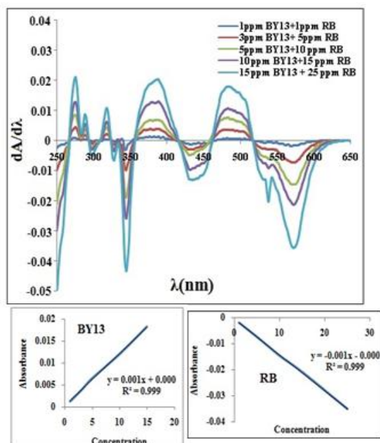
Fig.2. The calibration curve by using first-order absorption spectra for BY13 and RB in binary dye solutions.
