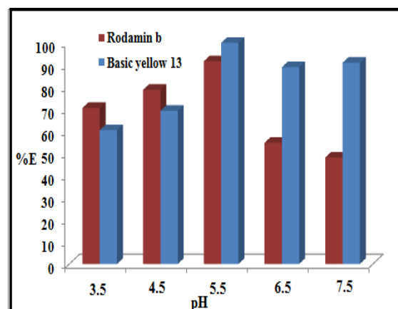
Fig.6. Effect of pH on photo-degradation of RB and BY13. Conditions: 100 mL mixture of two dyes with concentrations of 12 and 7 mgL -1 for RB and BY13, respectively; catalyst dosage, 5 mg; and irradiation time of 60 min.
