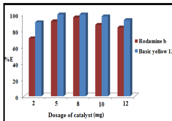
Fig.8. Effect of catalyst dosage on degradation efficiencies. Experimental conditions: 100 mL mixture of two dye with concentrations of 12 and 7 mgL -1 for RB and BY13, respectively, pH 5.5, irradiation time of 60 min.
