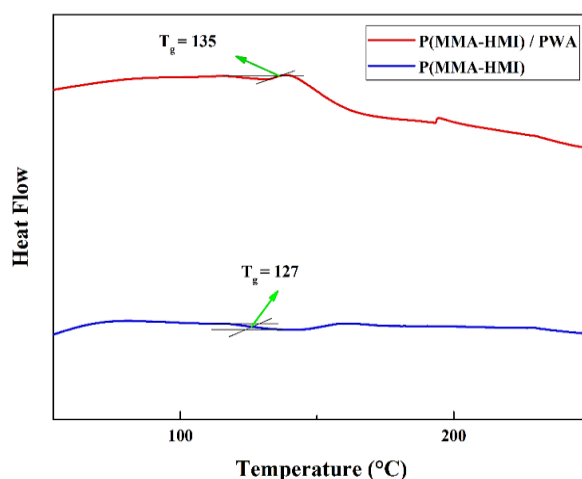
Fig. 8. DSC thermograms for (MMA-co-HMI)30 membrane and (MMA-co-HMI)30/PWA1.5 composite membrane
