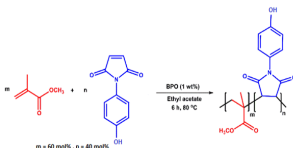
Fig. 3. Synthesis of poly(MMA-co-HMI) copolymer
