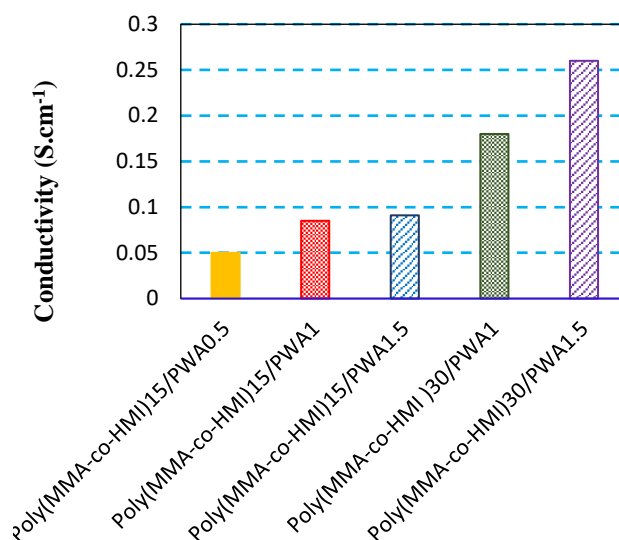
Fig. 10. Proton conductivity of poly(MMA-co-HMI)15 fabricated with different concentrations of PWA
