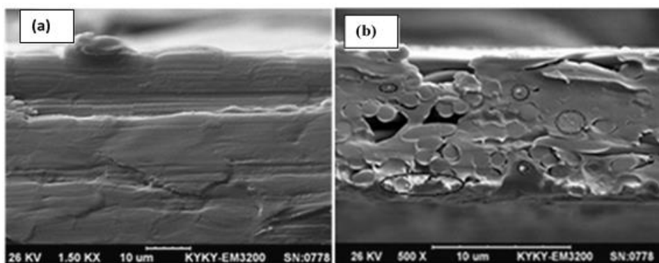
Fig. 11. SEM cross-section micrographs of (a) poly(MMA-co-HMI)30 and (b) poly(MMA-co-HMI)30/PWA1.5 membranes
