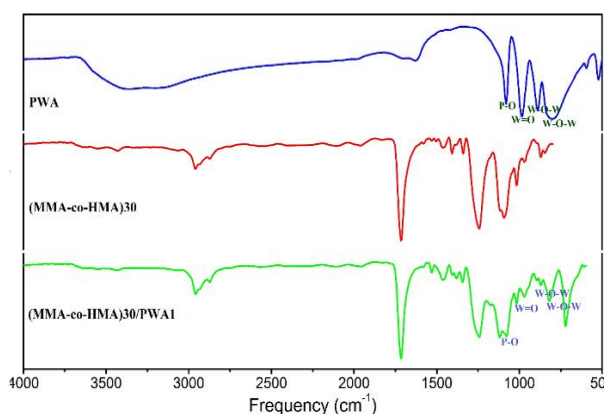
Fig. 5 FTIR spectra of PWA, poly(MMA-co-HMI)30 and poly(MMA-co-HMI)30/PWA1 membranes
