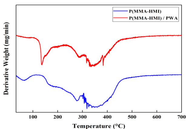
Fig. 6 TGA curves of the (MMA-co-HMI)30 membrane and (MMA-co-HMI)30 /PWA1.5 composite membrane
