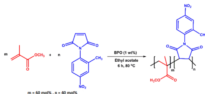
Fig. 1 Structure of poly(MMA-co-NMI) copolymer
