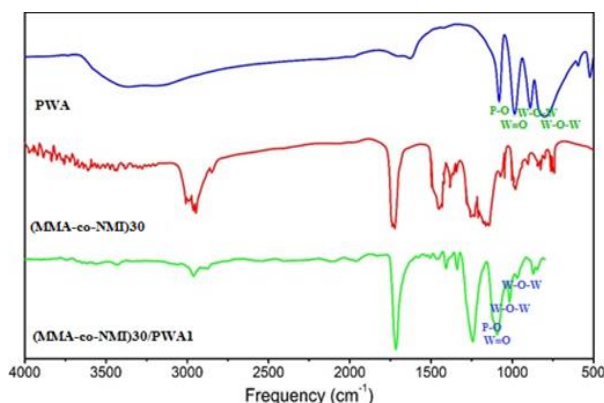
Fig. 4 FTIR spectra of PWA, poly(MMA-co-NMI)30 and poly(MMA-co-NMI)30/PWA1 membranes
