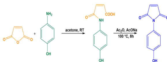
Fig. 2 Synthesis of N-4-hydroxyphenyl maleimide
