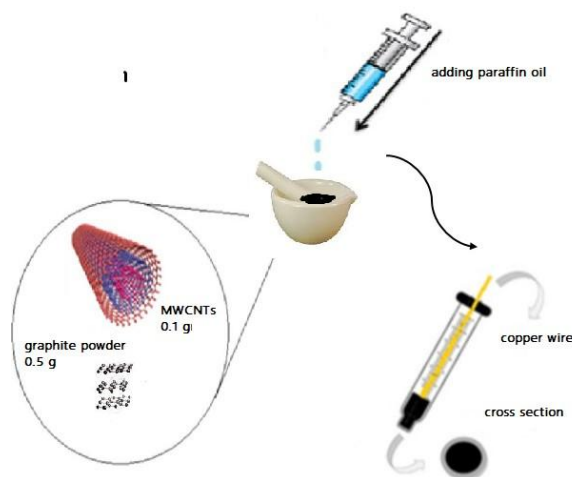
Fig.2. schematic representation of the steps preparation of MWCNTs-CPE
