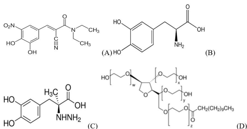
Fig. 1. Chemical structures of entacapone (A), levodopa (B), carbidopa(C), Tween 20(D)
