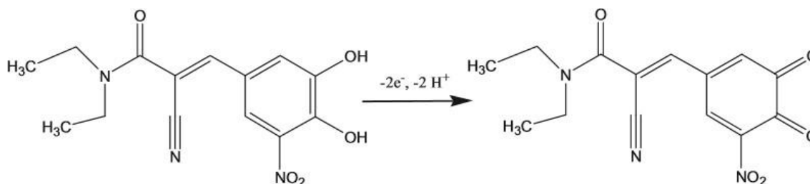
Fig. 5. The oxidation mechanism of ENT.
