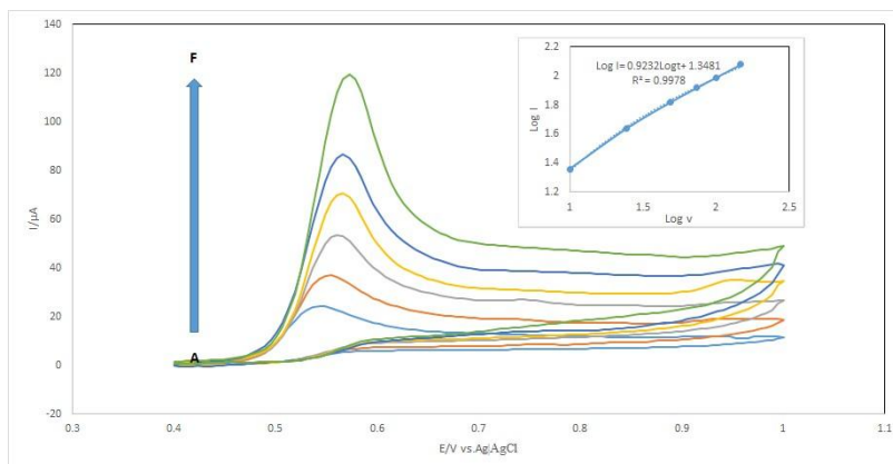
Fig.8. Cyclic voltammograms of ENT as a function of scan rate in presence of T20 at MWCNTs-CPE. The inset: the linear relationship between \log I and \log v in BR buffer of pH 2.0.
