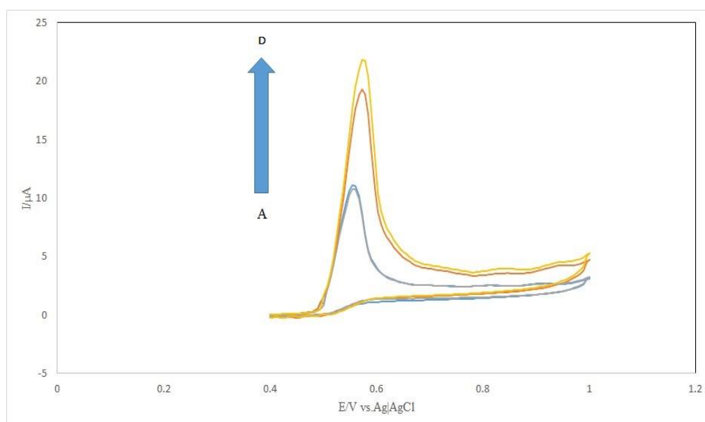
Fig. 7. Cyclic voltammograms of ENT in presence of CTAC (A), CTAB(B), SDS (C) and T20(D) in BR buffer of pH 2.0.
