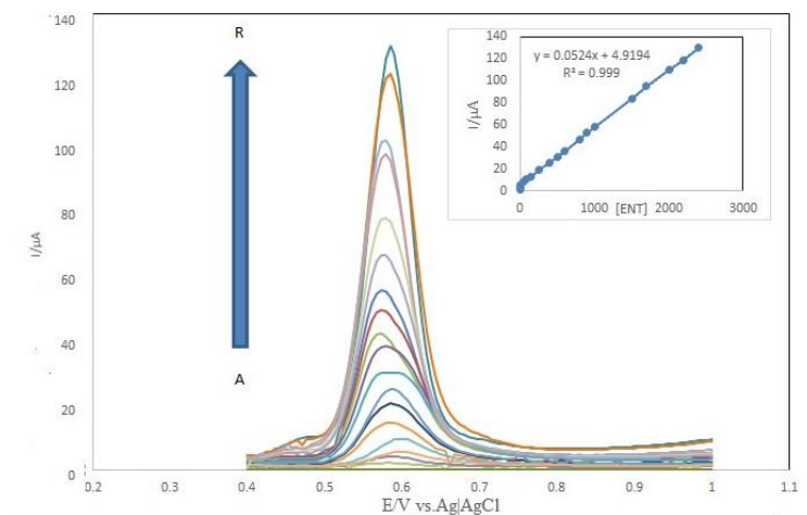
Fig .9. DPVs of ENT at MWCNTs-CPE in 0.1 M PBS. ENT concentration from down to up: 0.05, 3, 10, 50, 80, 150, 250, 400, 500, 600, 800, 900, 1000, 1500, 170, 2000, 2200 and 2400 \mu\text{M} .
