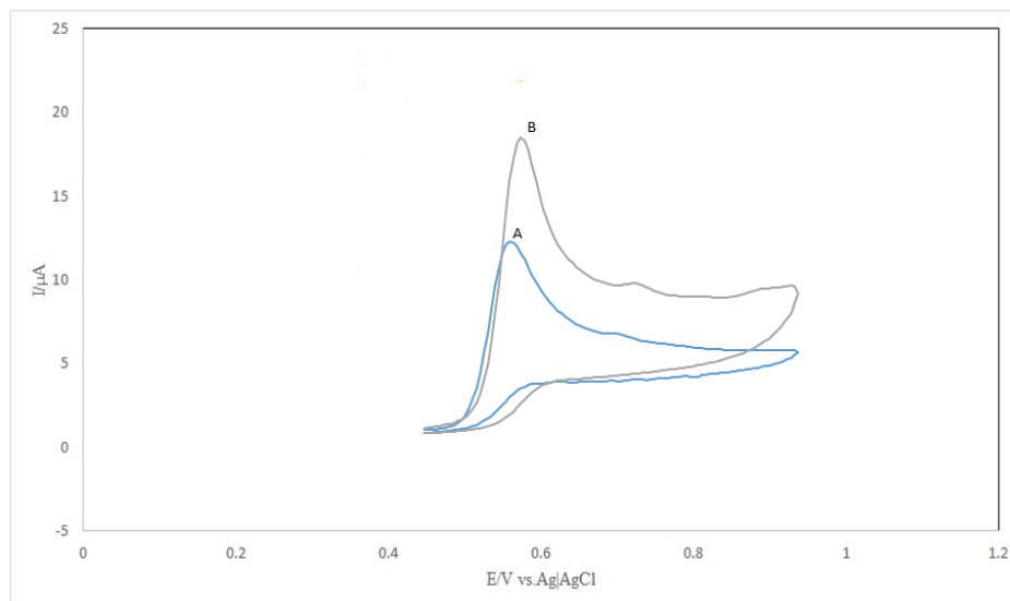
Fig. 4. Cyclic voltammogram of ENT in BR buffer of pH 2.0 at CPE(A) and MWCNTs-CPE(B)
