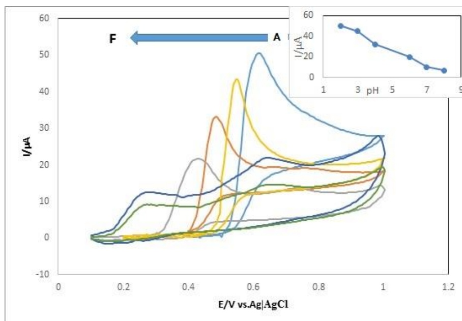
Fig.6. Effect of solution pH on the oxidation of 1000 \mu\text{M} ENT at MWCNTs-CPE; scan rate 100 mV/s. pH=A) 2.0, B)3, C)4, D)6, E)7 and F)8. The inset: the linear relationship between pH and I.
