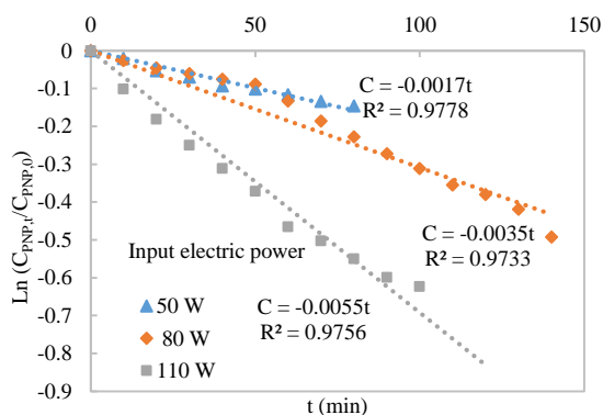
Fig. 3. Effect of input electric power to ultrasonic transducers on \ln(C_{\text{PNP},t}/C_{\text{PNP},0}) vs. time, pH:5, C_{\text{PNP},0} : 100 mg/L.
