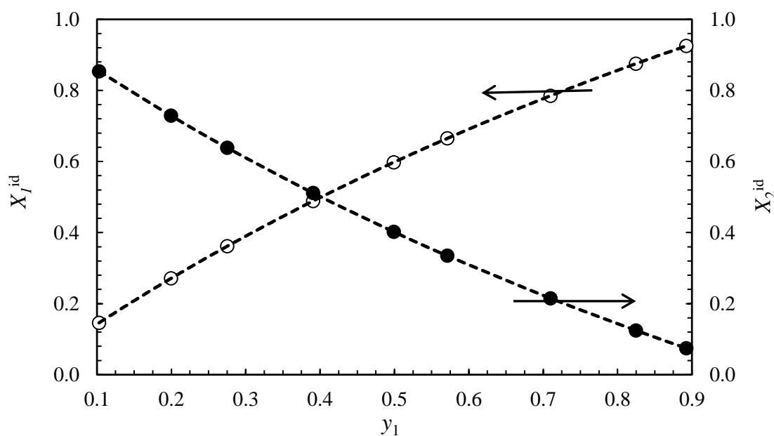
Fig. 6: Plot of the mole fractions of IL( X_1^{id} ) and DTAB( X_2^{id} ) as a function of the bulk mole fraction of IL ( y_1 ), in the mixed micelles of IL(1)/DTAB(2). The symbols refer to the calculated data by the ideal state model, and the continuous dashed curve is a guide for the eyes.
