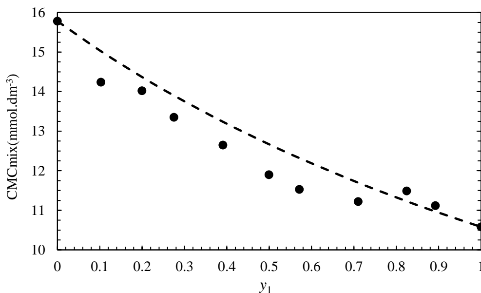
Fig. 5: Plot of critical micelle concentration, CMC, as a function of the bulk mole fraction of IL( y_1 ), in the mixtures of IL(1)/DTAB(2). The symbols refer to the experimental data, and the continuous dashed curve represents the calculated values with Clint's theory.
